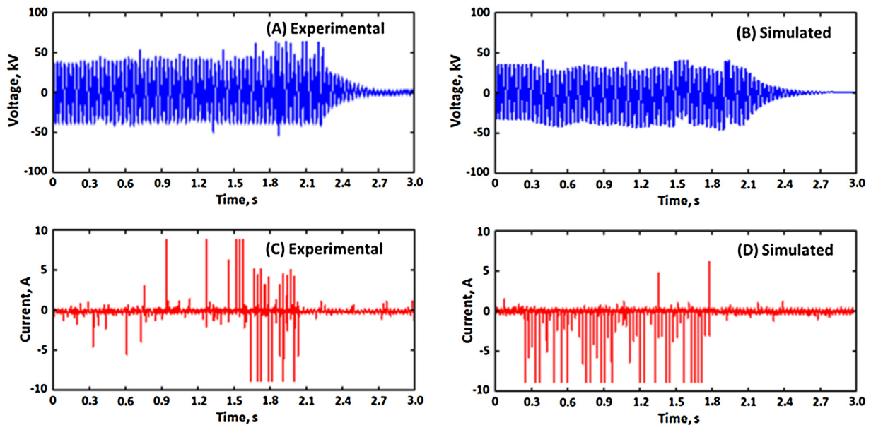
Fig. 10. All discs polluted, 60 g salt and 160 g kaolin.
