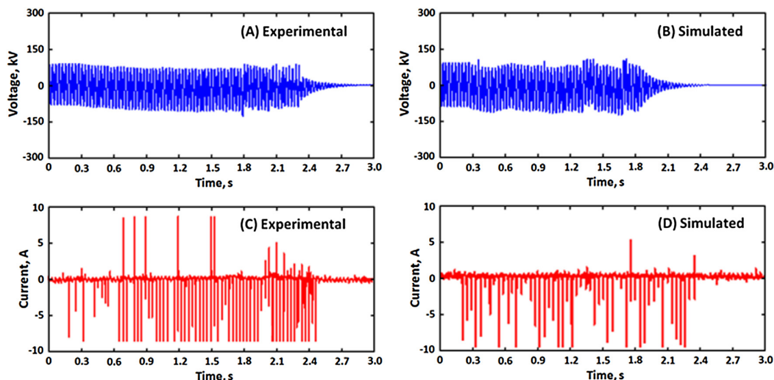
Fig. 8. Two polluted discs, 60 g salt and 160 g kaolin.
