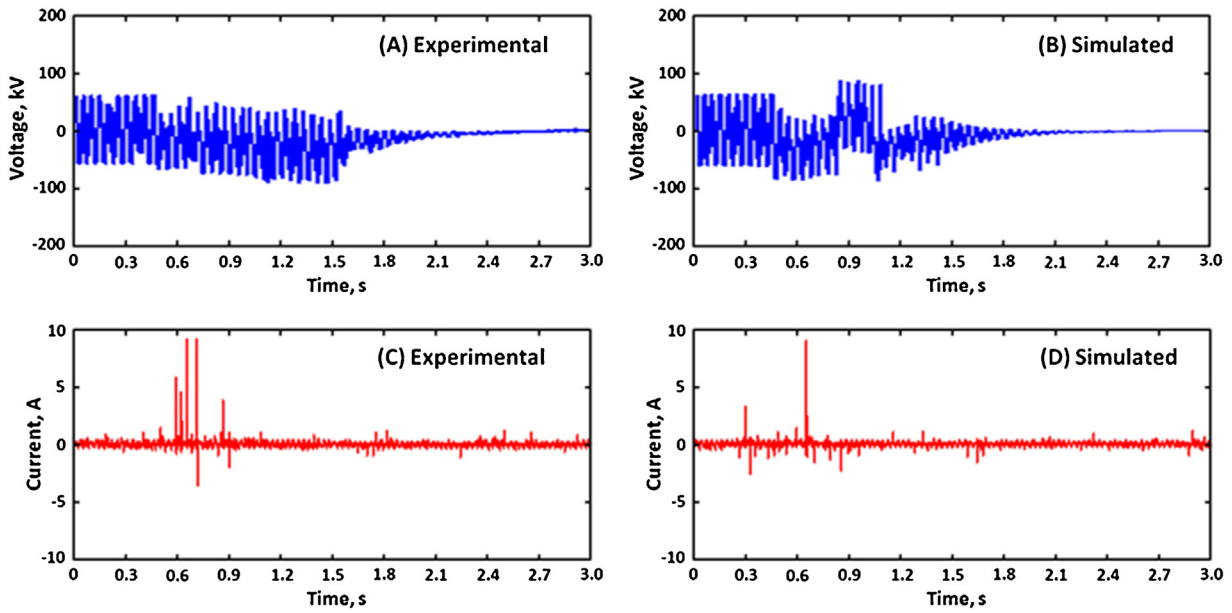
Fig. 9. Four polluted discs, 60 g salt and 160 g kaolin.
