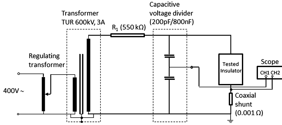
Fig. 2. Connection of test circuit.
