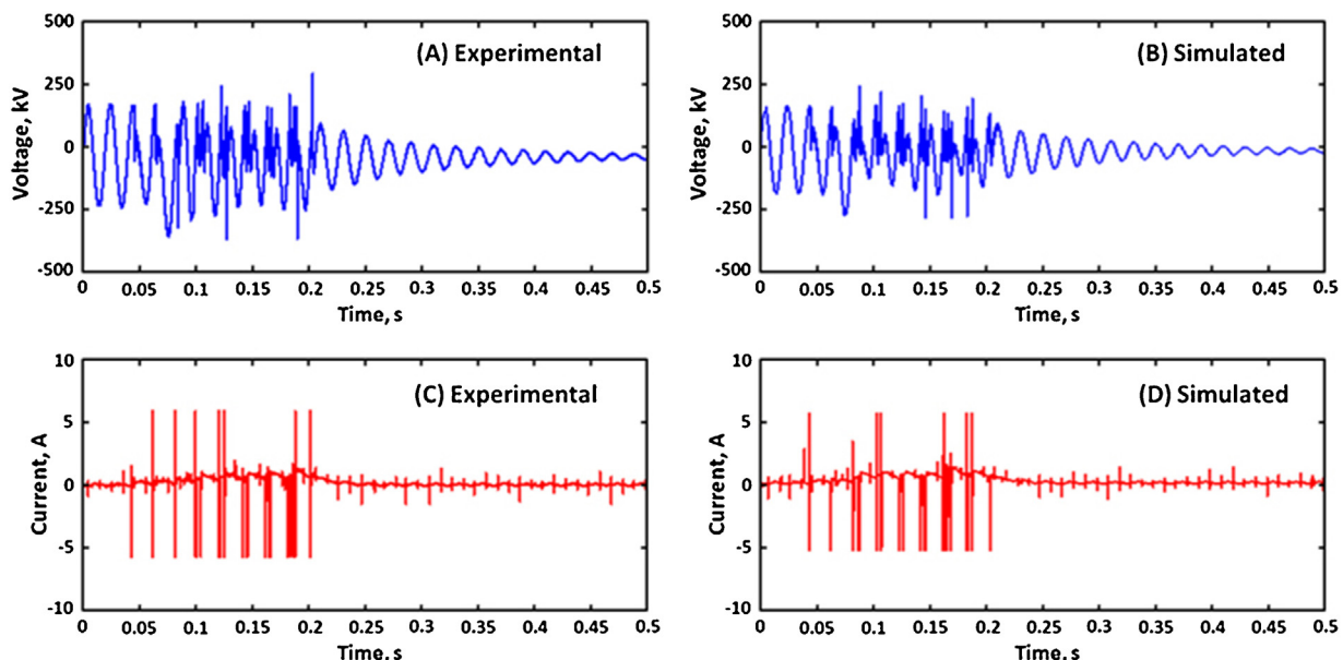
Fig. 5. Two polluted discs, 15 g salt and 40 g kaolin.
