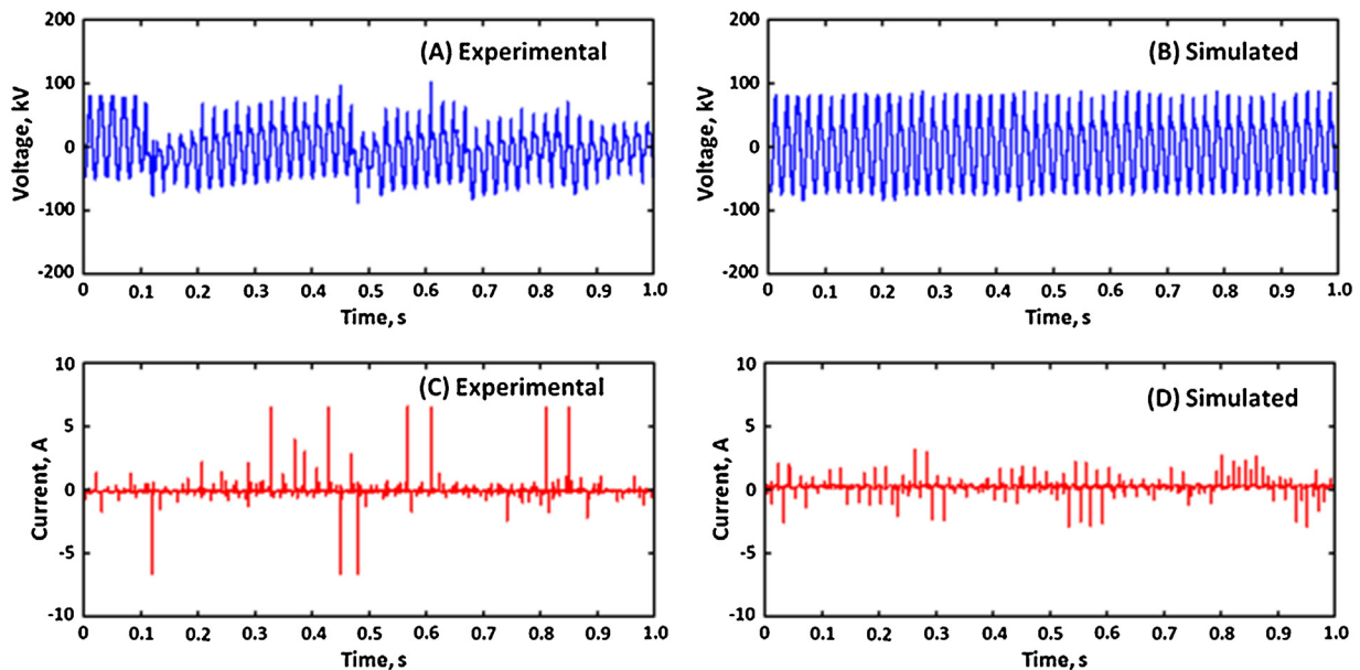
Fig. 7. All discs polluted, 15 g salt and 40 g kaolin.
