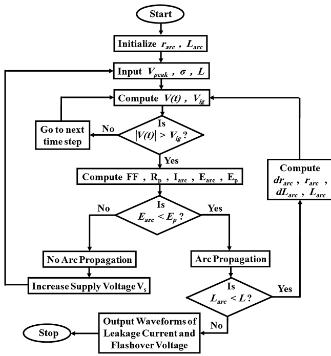
Fig. 3. Flow chart of dynamic arc model with AC energization.
