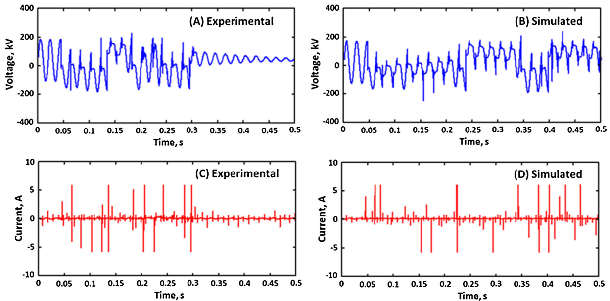
Fig. 6. Four polluted discs, 15 g salt and 40 g kaolin.
